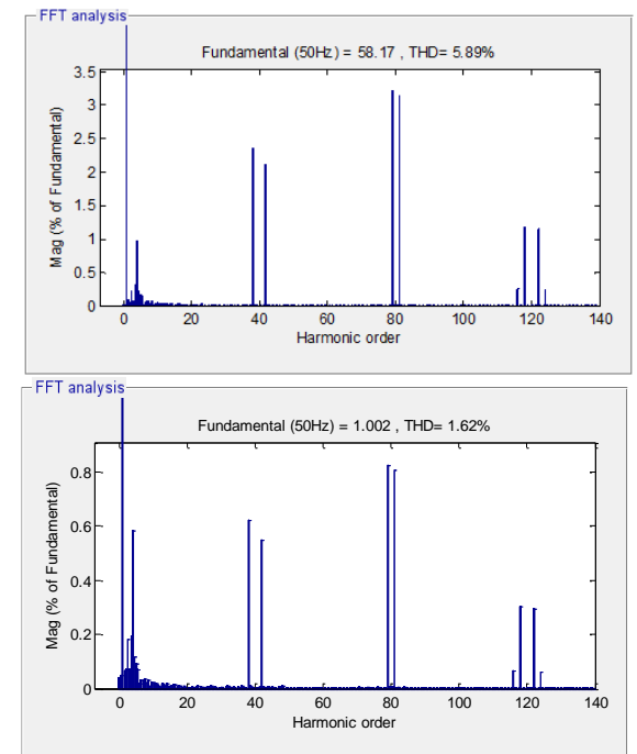
Fig. 12. Output voltage and current THD
