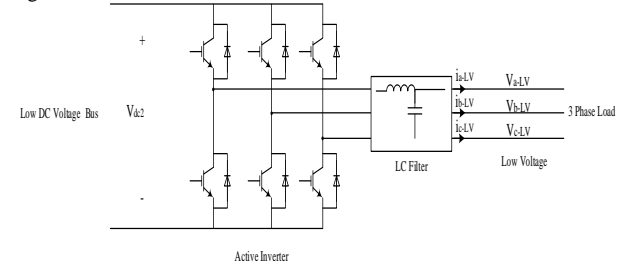
Fig. 6. The conventional inverter schematic.
