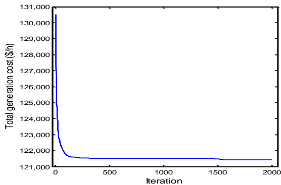
Fig. 1. The convergence characteristic of fuel cost
